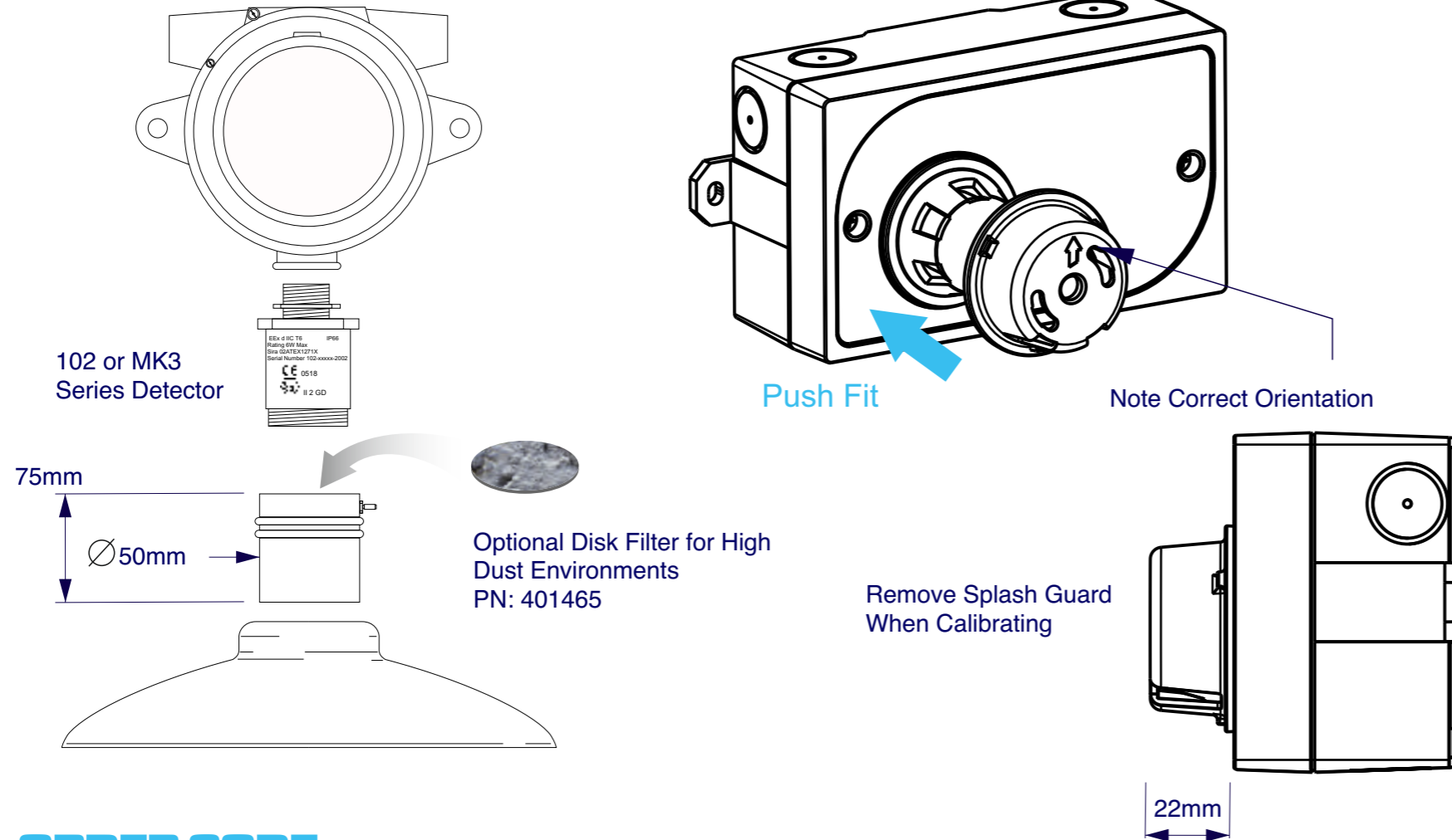
TOC-750-GD1 Splash Guard
